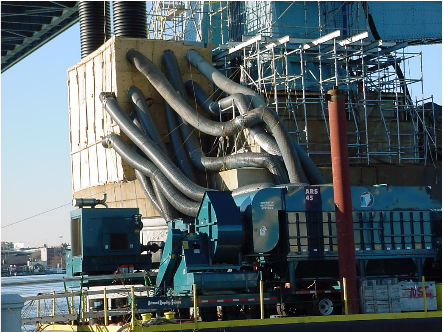
Ben Franklin Bridge Tower – Exhaust Ducts From Dust Collector
